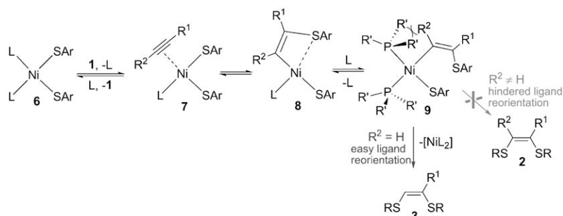
Scheme 6. C–S reductive elimination by means of the ligand dissociative pathway ( L = \text{PPh}_3 ).
