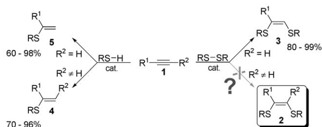
Scheme 1. Transition-metal-catalyzed S-S and S-H bonds addition to alkynes.
