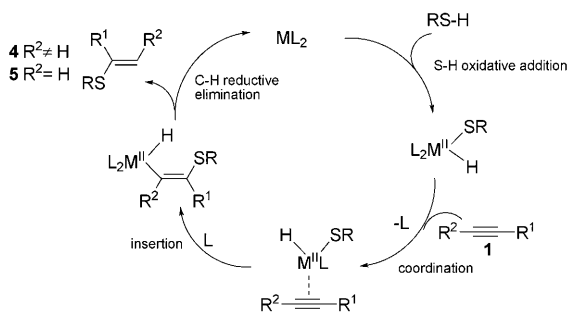
Scheme 2. The mechanism of the catalytic S-H bond addition to terminal and internal alkynes. [9,10]
