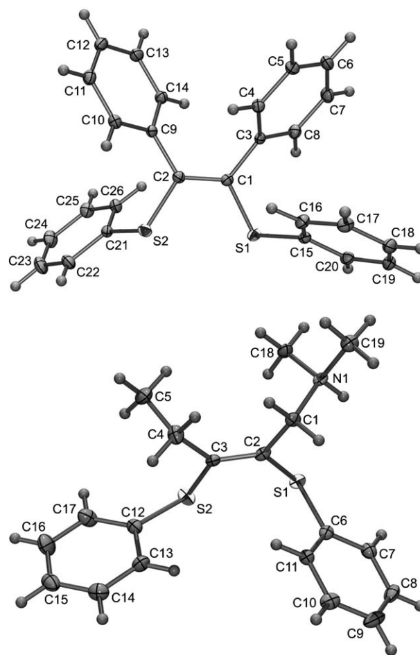
Figure 1. X-ray structures of 2d (top) and 2e (bottom; only one of the two crystallographically independent cations is shown).
