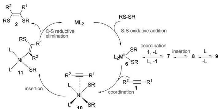
Scheme 7. C-S reductive elimination through the apical site of the metal without ligand dissociation ( L = \text{PMePh}_2 ).
