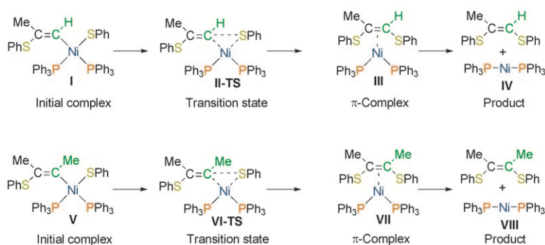
Scheme 5. The model system for theoretical study of C–S reductive elimination reaction involving \alpha -unsubstituted vinyl group (top) and \alpha -Me-substituted vinyl group (bottom); C–H and C–Me groups in \alpha -position are highlighted with green color. [28]
