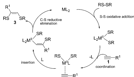
Scheme 3. The mechanism of the catalytic S-S bond addition to terminal alkynes. [10]
