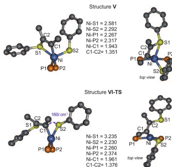
Figure 2. The structures of V and VI-TS optimized at PBE/TZP level (some atoms are omitted for clarity [28] ); selected bond lengths are given in Å.
